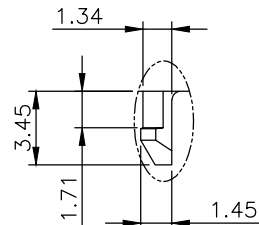
DETAIL Z SCALE 2:1
