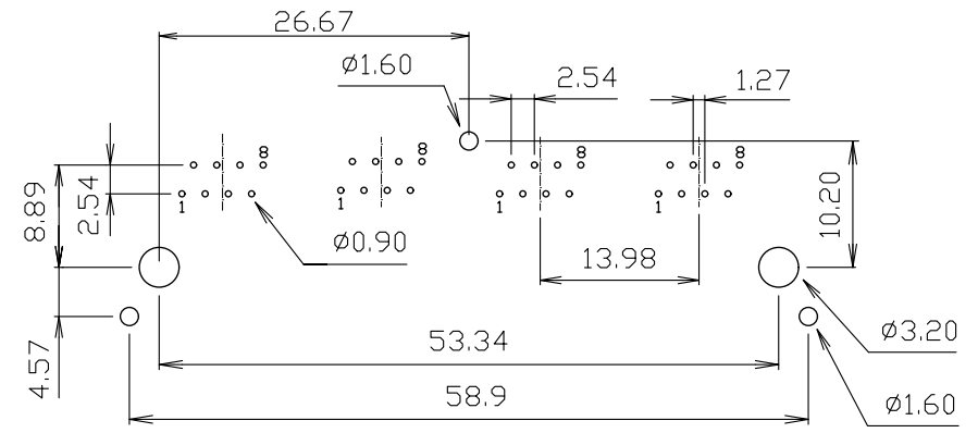
PC Board Layout Ref.
