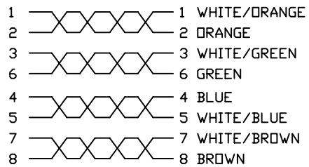
PINOUT DIAGRAM:
