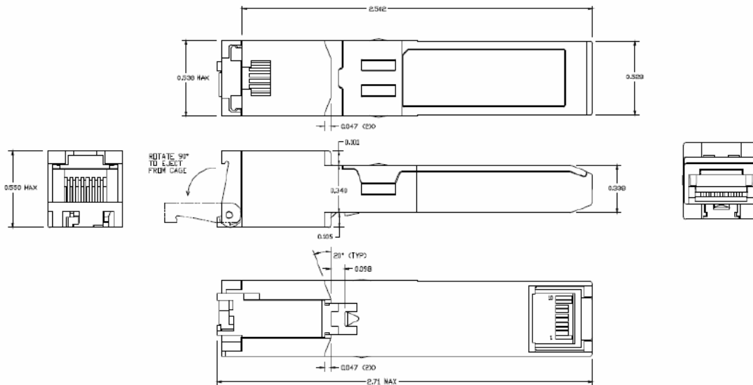
Figure 2. XSFP-T-PXRC mechanical dimensions
