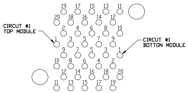
CONNECTOR PIN-OUT COMPONENT SIDE OF BOARD
