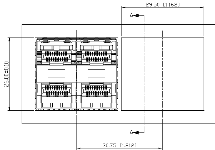
BEZEL CUT-OUT CENTER SPACING DETAIL BEZEL THICKNESS: 0.8-2.6
