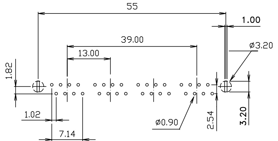
SUGGESTED PCB LAYOUT TOP VIEW PCB LAYOUT TOLERANCE .XX±0.05[0.002]
