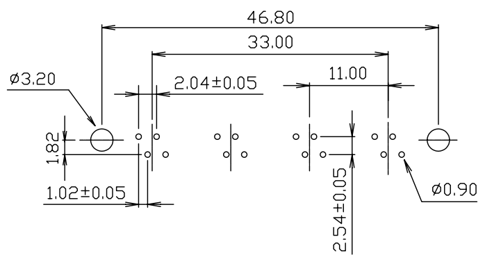
SUGGESTED PCB LAYOUT (TOP VIEW)
