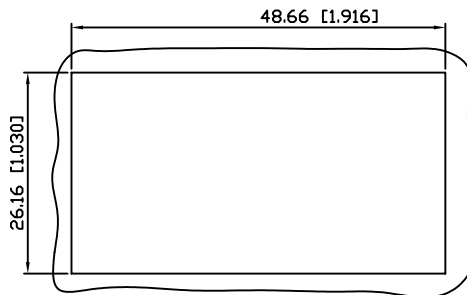
RECOMMENDED PANEL CUTOUT DIMENSION
