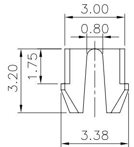
DETAIL X
