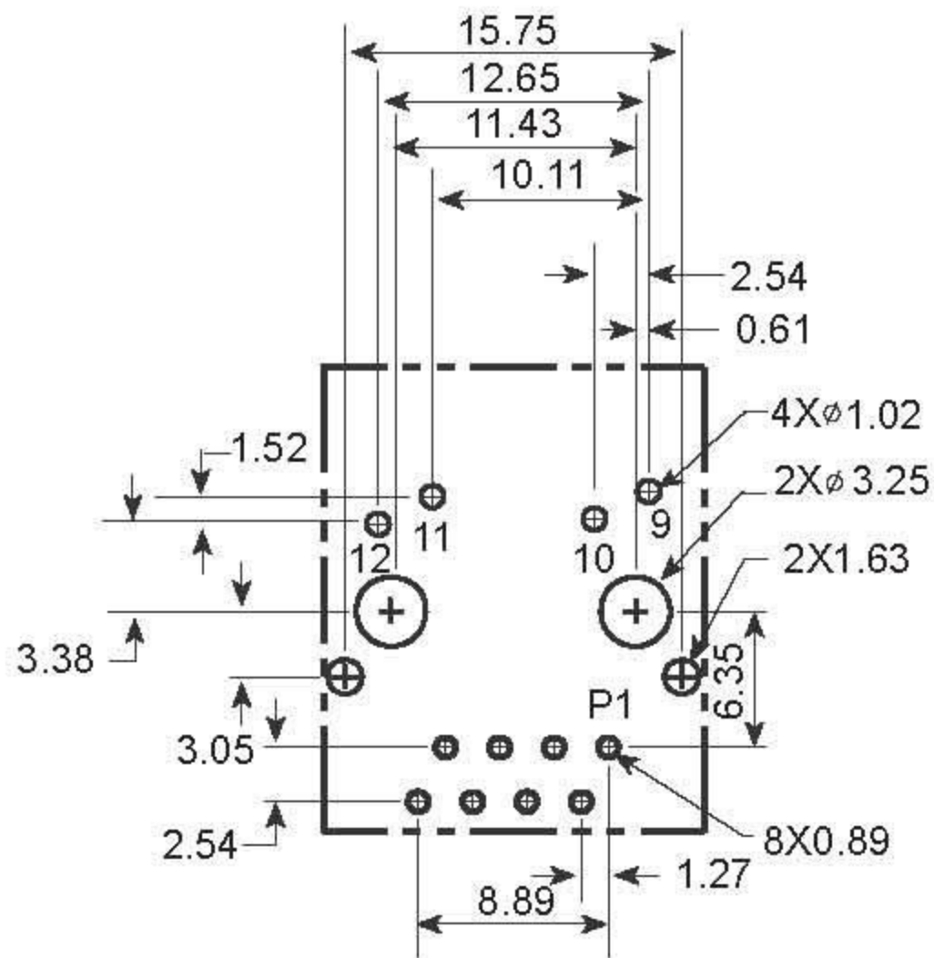
Viewed from PCB Component side
