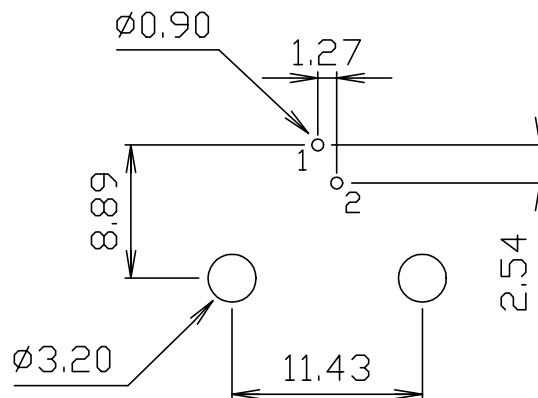
SUGGESTED PCB LAYOUT TOLERANCE .XX±0.05[0.002]
