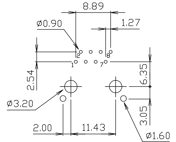
SUGGESTED PCB LAYOUT PCB LAYOUT TOLERANCE TOP VIEW .XX±0.05[0.002]
