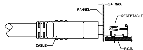
REFERENCE MOUNT DIMENSION
