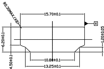
REFERENCE PANEL CUT OUT DIMENSION
