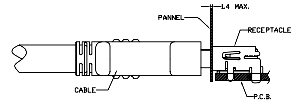
REFERENCE MOUNT DIMENSION
