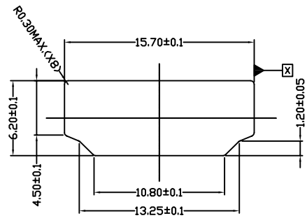
REFERENCE PANEL CUT OUT DIMENSION
