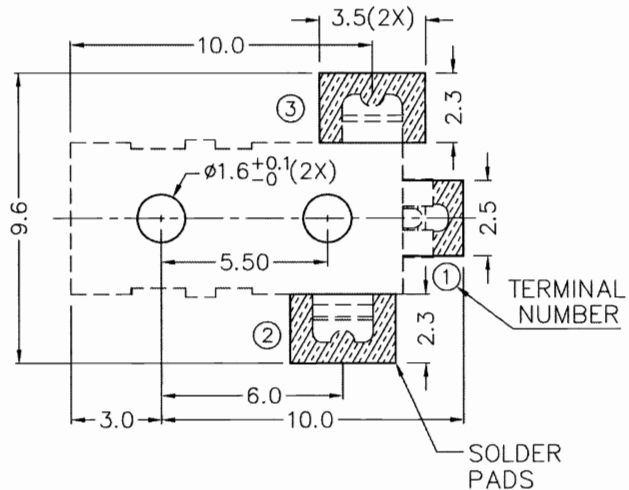
RECOMMENDED SOLDER PAD LAYOUT
