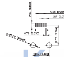
SUGGESTED PCB LAYOUT TOP VIEW
