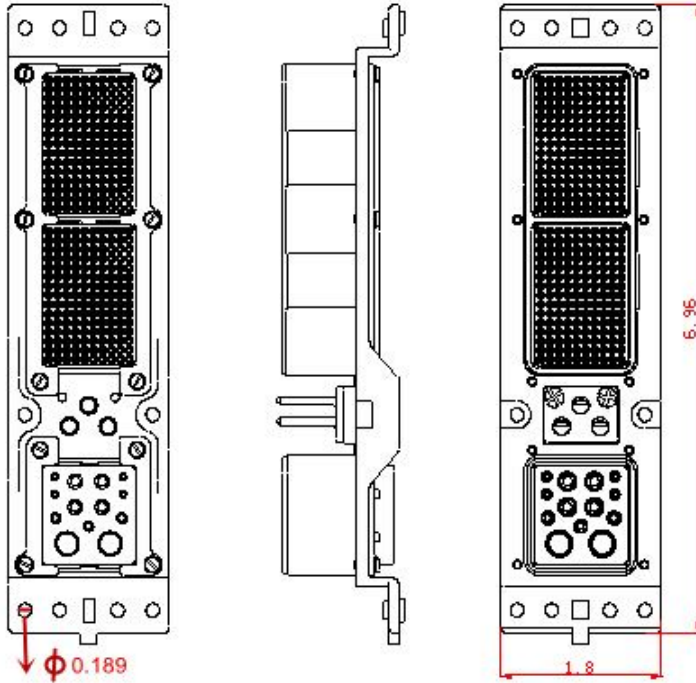
DIMENSION
